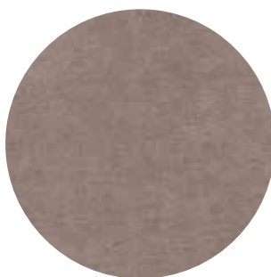
liver 10
